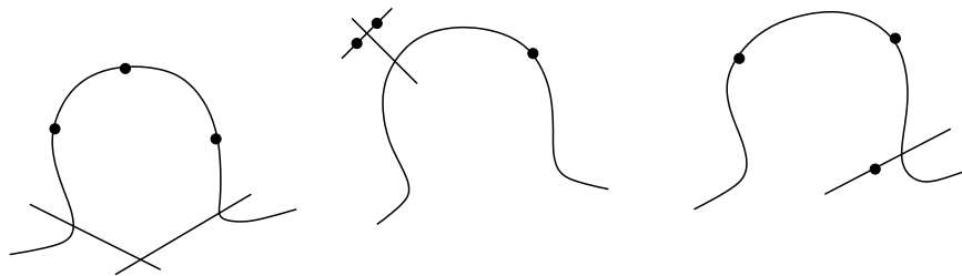
Figure 3.1: Examples of 3-pointed semistable curves which are NOT quasistable
