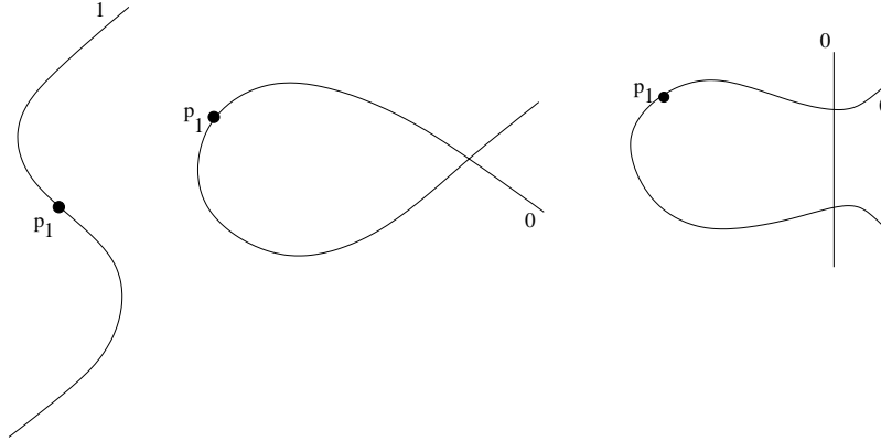
Figure 3.2: 1-pointed quasistable curves of genus 1.
