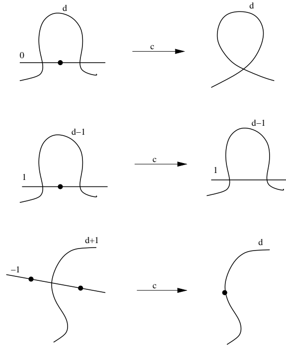
Figure 3.4: Contractions of quasistable pointed curves over k and balanced degree d line bundles.
