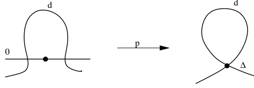
Figure 3.5: Stabilization of pointed quasistable curves with balanced degree d line bundles.
