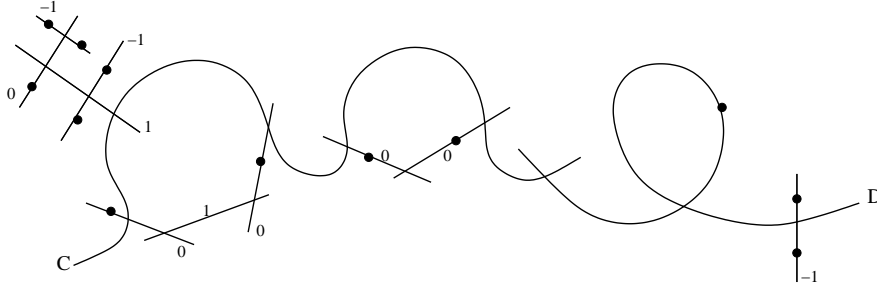
Figure 3.3: 12-pointed quasistable curve with assigned balanced multidegree in rational tails and rational bridges.
