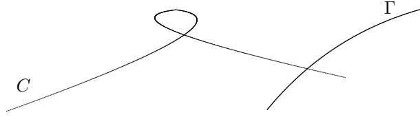
FIGURE 9. The special fibers of f : X \rightarrow \mathbb{P}^1 .
