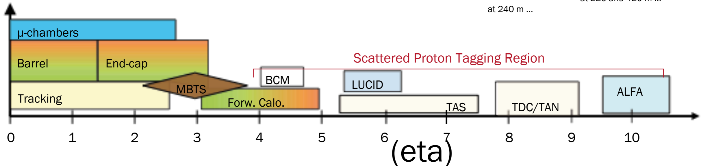
BCM [Beam Condition Monitor] Diamond sensors at z = \pm 184 cm 4 modules per side
