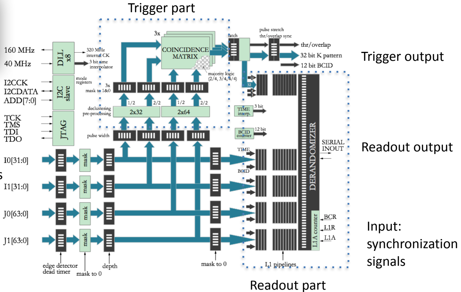
Coincidence Matrix ASIC for Muon Trigger in the Barrel of ATLAS
